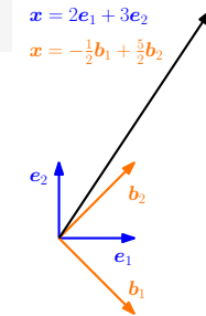
Figure 2.9 Different coordinate representations of a vector x , depending on the choice of basis.
